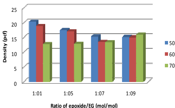
Fig. 1 Density of Polyurethane Each bar representing the temperature reaction: 50,60, and 70°C
