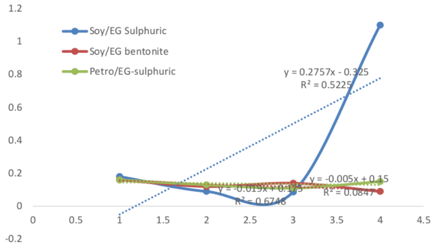
Figure 8. Comparing the Density to Petro based Polyol
