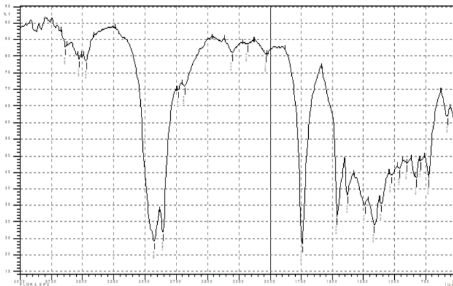
Figure 4. FTIR images of Soy epoxide
