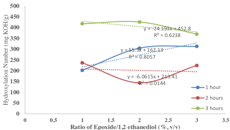
Figure 3. The optimized of soy-polyol
