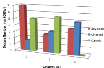
Fig. 1. Catalyst for epoxidation at 60°C
