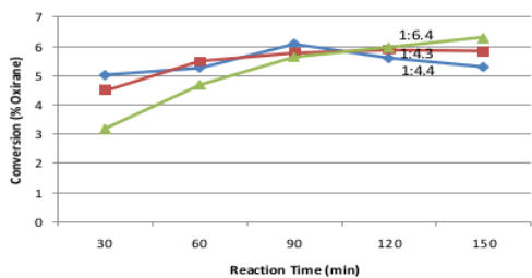
Fig. 4 Oxidation with peracetic acid at 50 0 C. The concentration was a ratio of acetic acid to H 2 O 2
