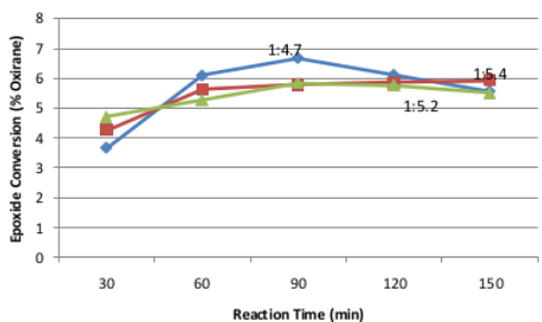
Fig. 5. Oxidation with peracetic acid at 60 0 C. The concentration was a ratio of acetic acid to H 2 O 2
