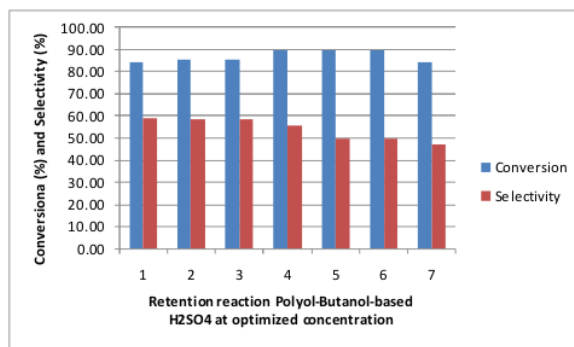
Figure 4. Epoxidation of Butanol-based with H_2SO_4
