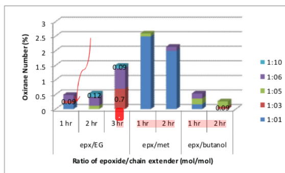
Figure 1. Time of reaction Optimization
