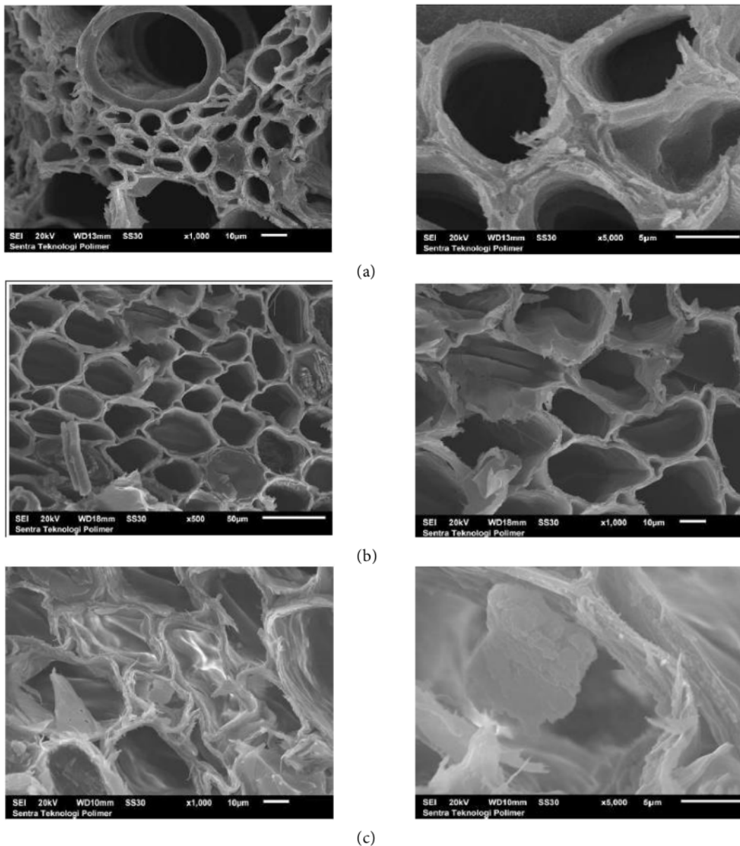
Figure 1. Scanning electron microscopy tensile fracture surface of soybean with 25% of alkali treatment a) Compression of surface of using canola with 25 % of alkali treatment b) Compression of plain bamboo fibre without matrix and alkali treatment.
