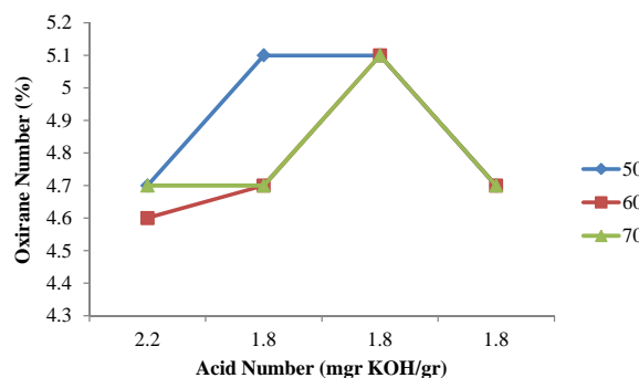
Figure 2. Oxirane Number as a Function of Temperature and Acid Number
