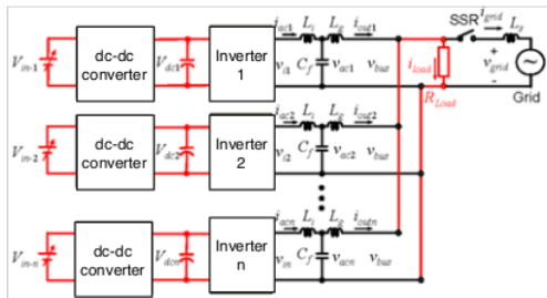
Figure 3. Configuration of distributed electric network
