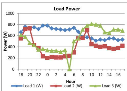
Figure 15. Power of inverter load
