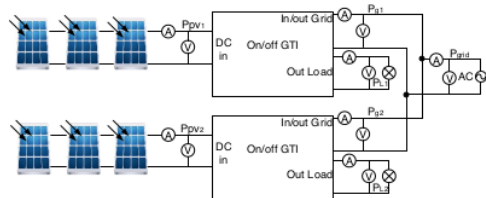
Figure 6. Circuit of on grid inverter
