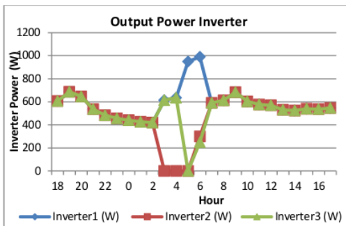
Figure 14. Inverter output power
