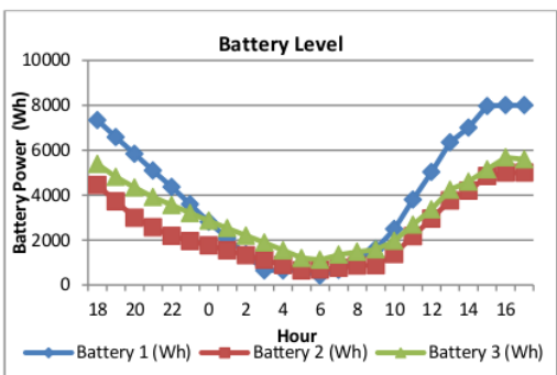
Figure 13. Battery Power Level
