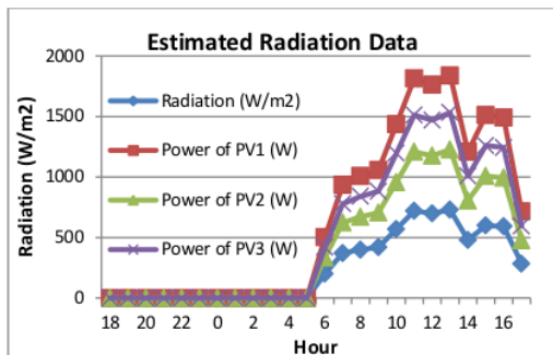
Figure 10. Data simulated radiation forecasts
