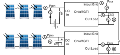
Figure 7. Circuit of parallel inverter in off grid/islanding
