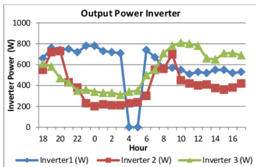
Figure 12. Graph output power of each inverter
