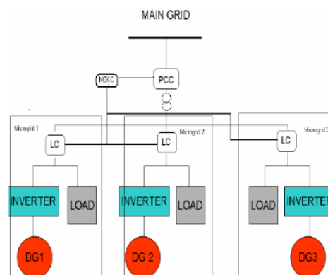
Figure 1. Diagram of microgrid system
