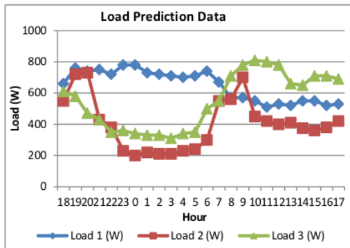
Figure 11. Simulation data load estimates
