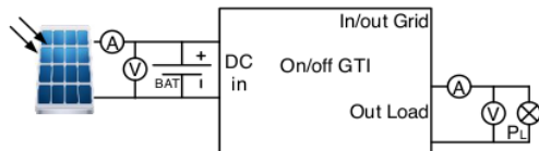
Figure 5. Circuit of stand alone/off grid inverter
