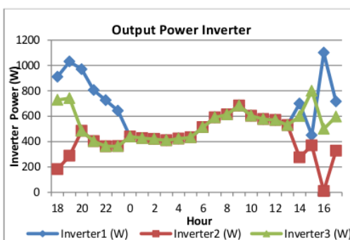
Figure 17. Output power inverter
