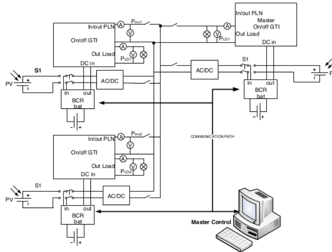
Figure 2. Diagram microgrid system using on / off GTI with power sharing control system during islanding conditions
