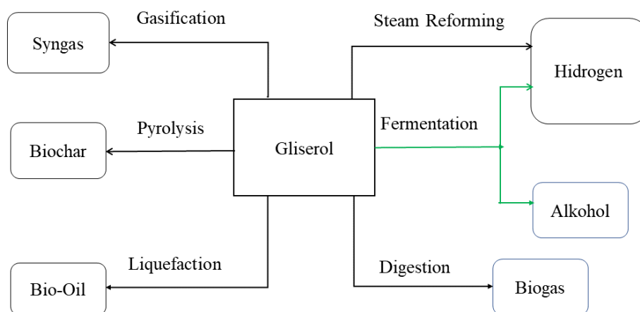
Figure 2. Diagram of Glycerol Conversion Pathway into Various Energy Products [29]
