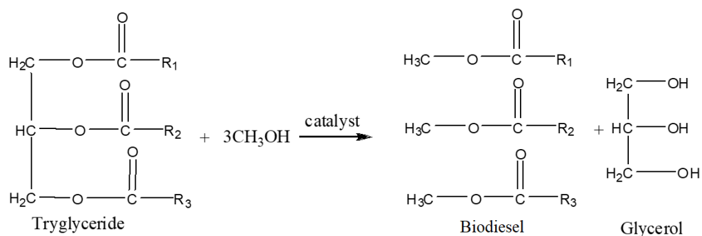
Figure 1. Transesterification Reaction Scheme [70]
